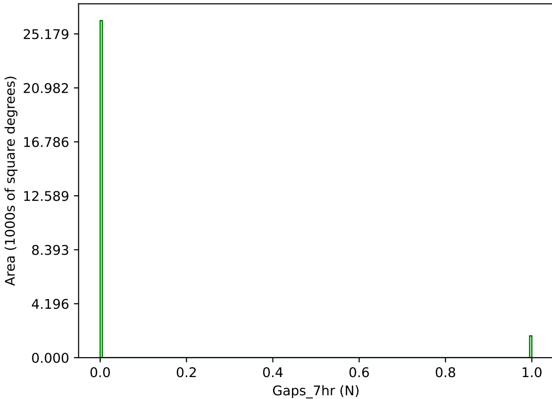
too_elab_r256_d3_gz_v3.4_10yrs g band: Gaps_7hr
