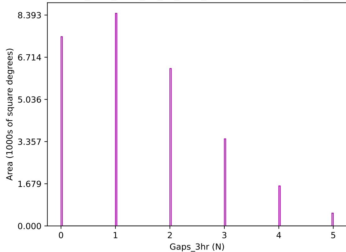
too_elab_r256_d3_gz_v3.4_10yrs z band: Gaps_3hr
