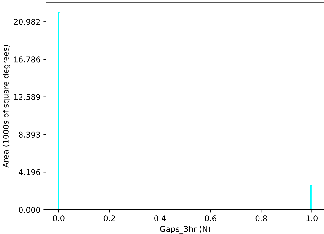
too_elab_r256_d3_gz_v3.4_10yrs u band: Gaps_3hr
