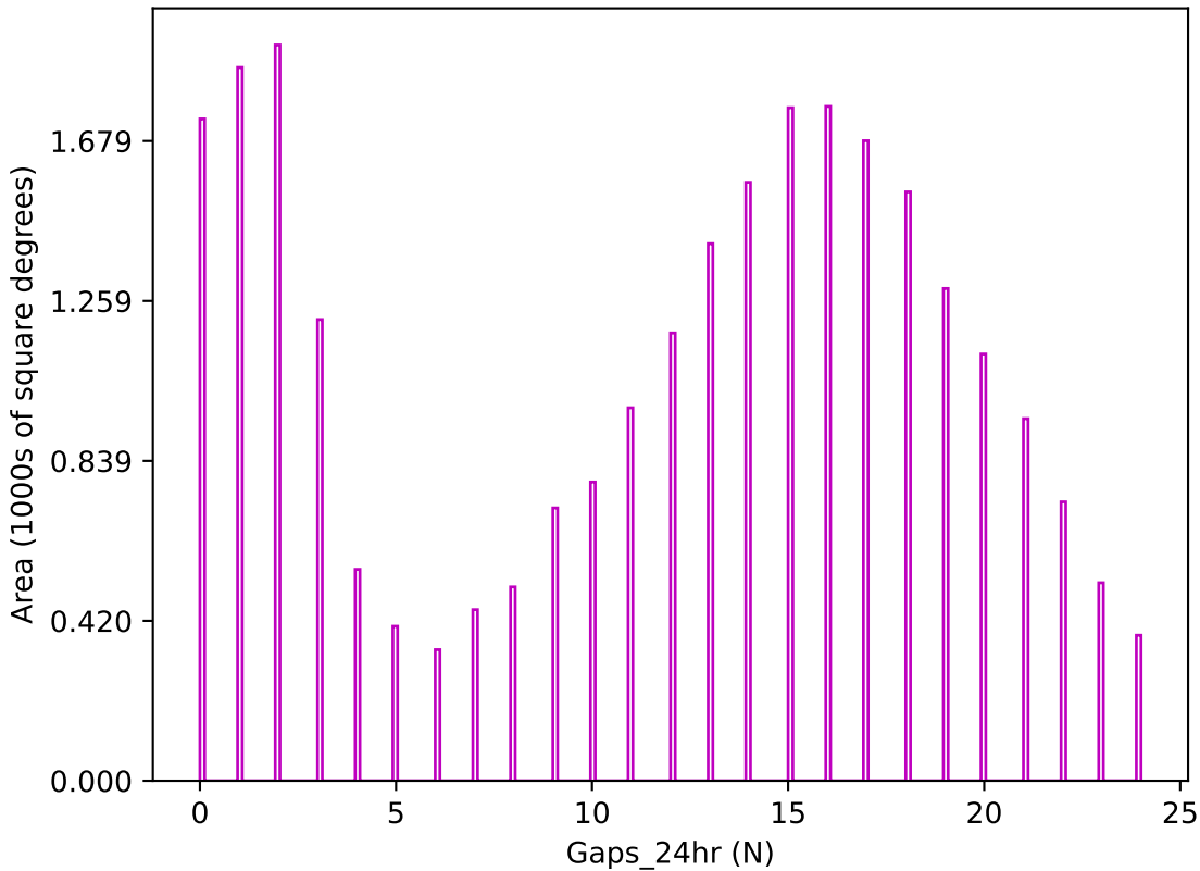
too_elab_r256_d3_gz_v3.4_10yrs z band: Gaps_24hr
