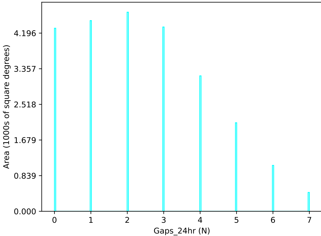
too_elab_r256_d3_gz_v3.4_10yrs u band: Gaps_24hr
