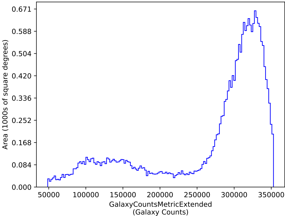
too_elab_r256_d3_gz_v3.4_10yrs y: GalaxyCountsMetricExtended
