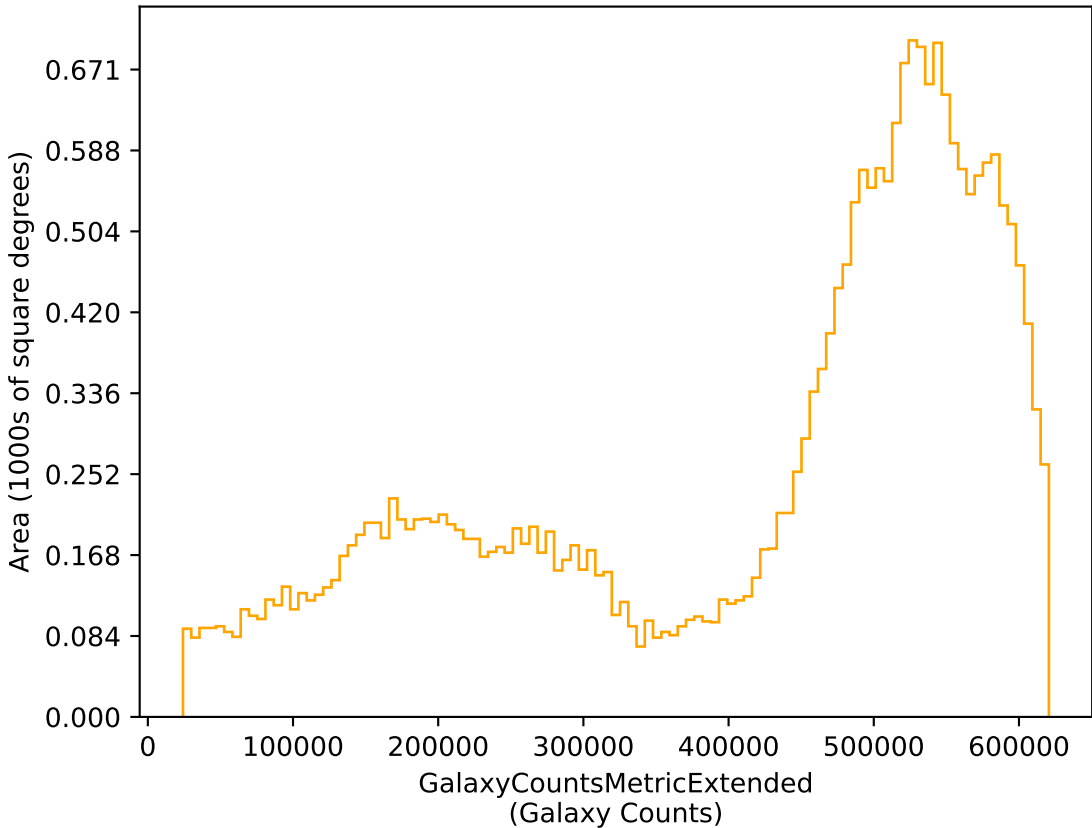
too_elab_r256_d3_gz_v3.4_10yrs r: GalaxyCountsMetricExtended
