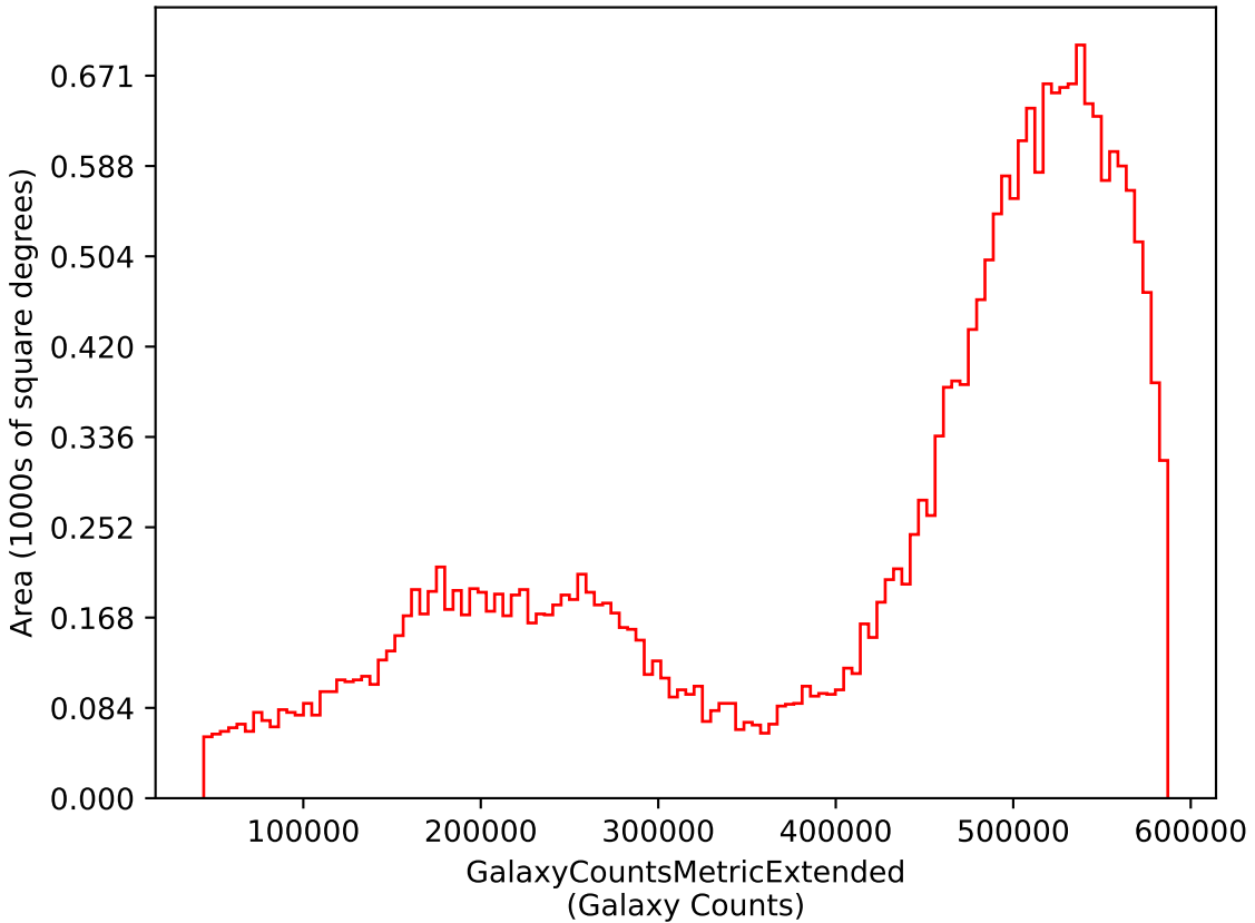
too_elab_r256_d3_gz_v3.4_10yrs i: GalaxyCountsMetricExtended
