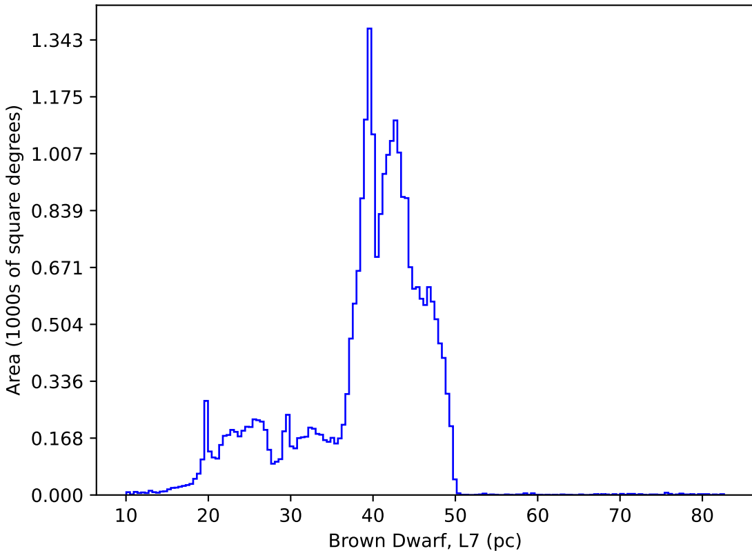
too_elab_r256_d3_gz_v3.4_10yrs : Brown Dwarf, L7
