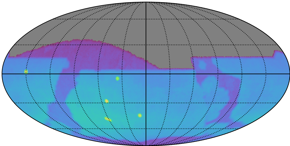
too_elab_r256_d3_gz_v3.4_10yrs : Brown Dwarf, L4
