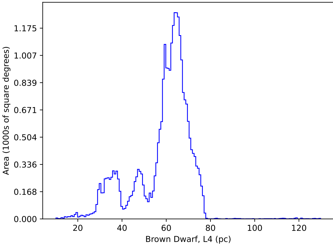
too_elab_r256_d3_gz_v3.4_10yrs : Brown Dwarf, L4
