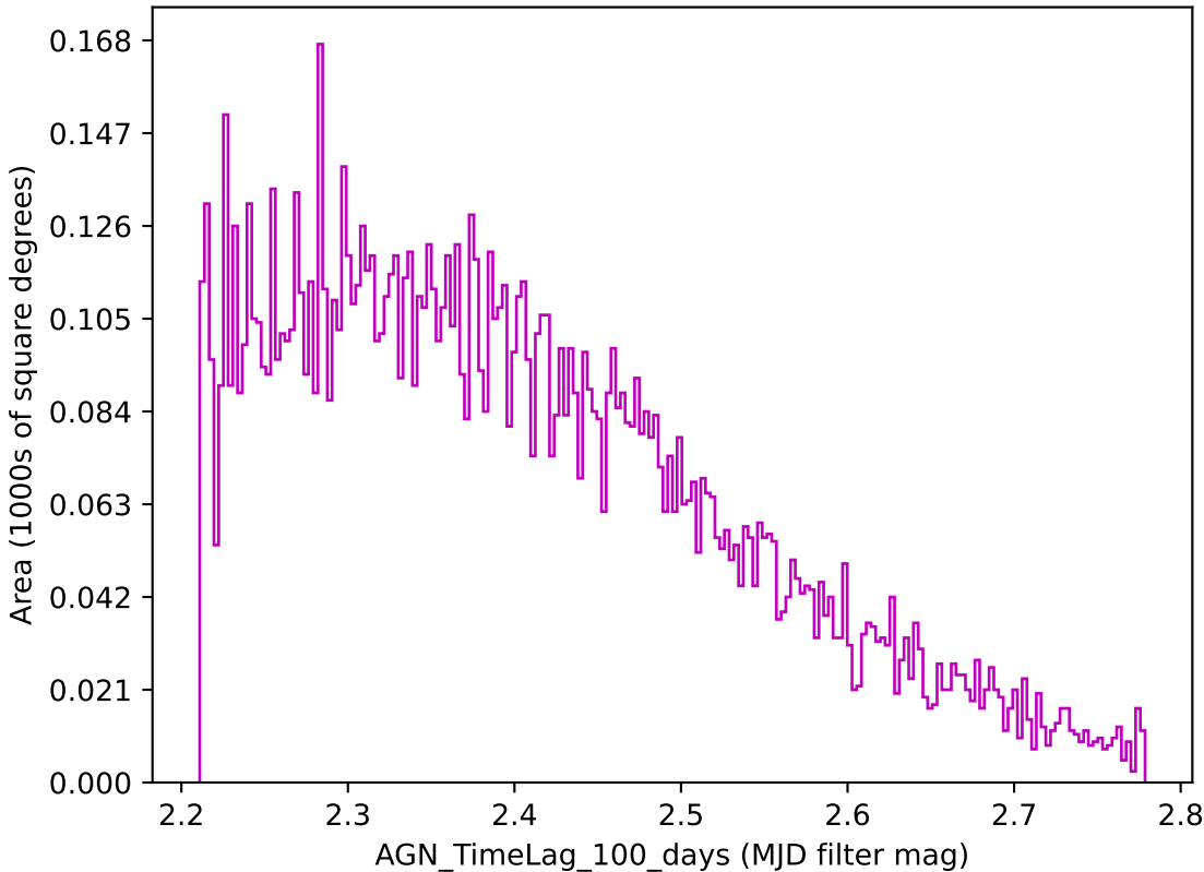
too_elab_r256_d3_gz_v3.4_10yrs z band: AGN_TimeLag_100_days
