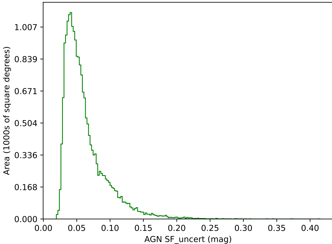
too_elab_r256_d3_gz_v3.4_10yrs g band: AGN SF_uncert
