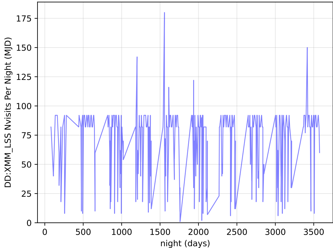
too_elab_r256_d3_gz_v3.4_10yrs all bands: DD:XMM_LSS Nvisits Per Night
