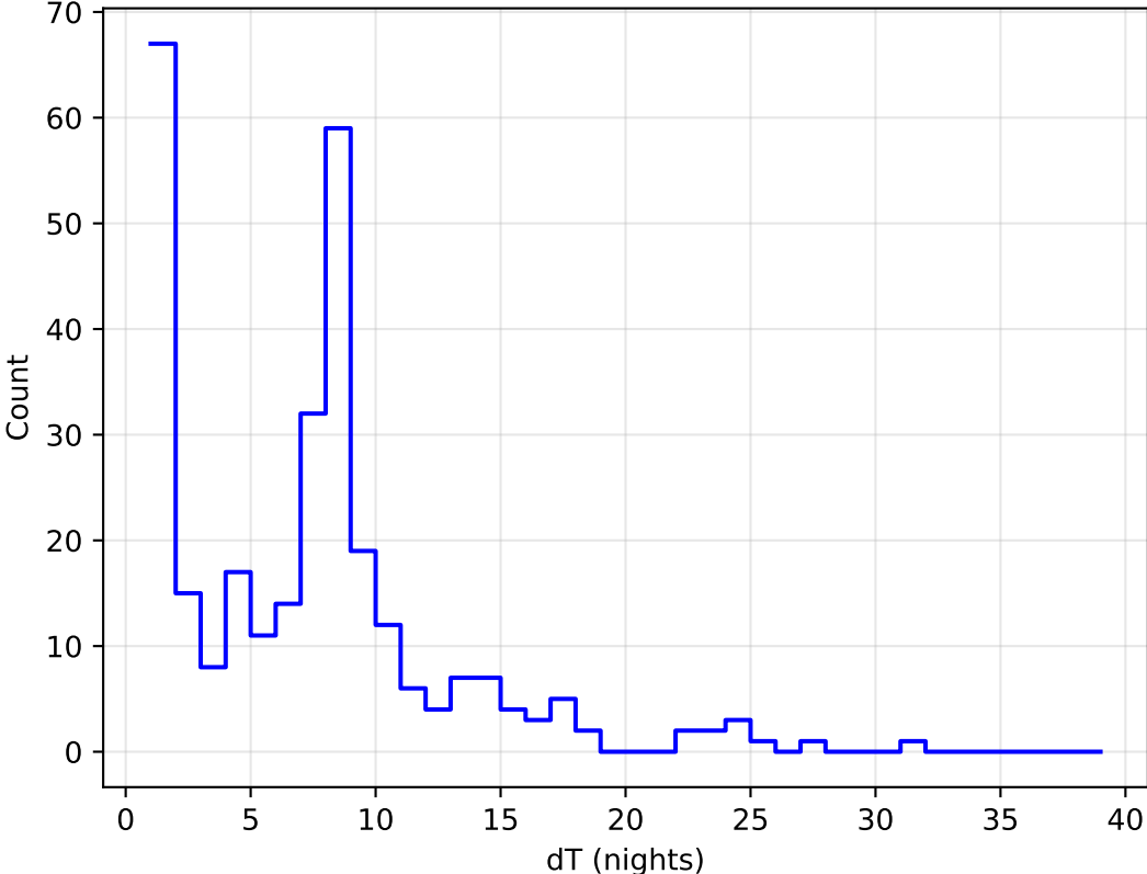
too_elab_r256_d3_gz_v3.4_10yrs all bands: DD:XMM_LSS Delta Nights Histogram
