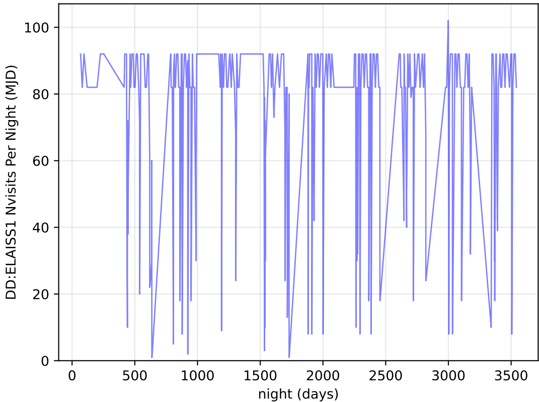
too_elab_r256_d3_gz_v3.4_10yrs all bands: DD:ELAISS1 Nvisits Per Night
