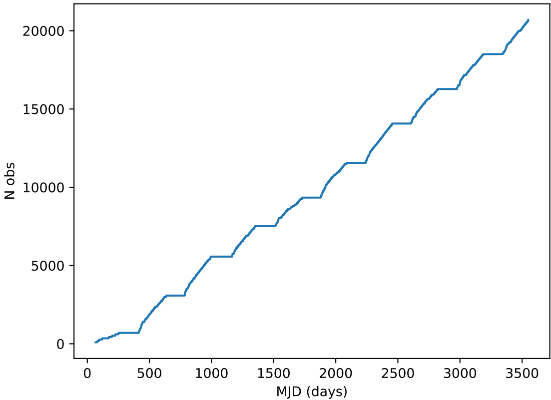
too_elab_r256_d3_gz_v3.4_10yrs all bands: DD:ELAISS1 Cumulative NVisits
