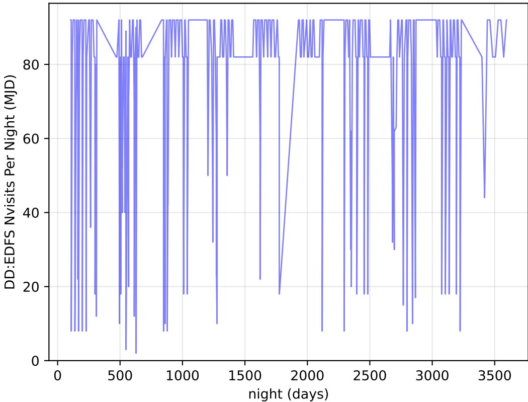
too_elab_r256_d3_gz_v3.4_10yrs all bands: DD:EDFS Nvisits Per Night
