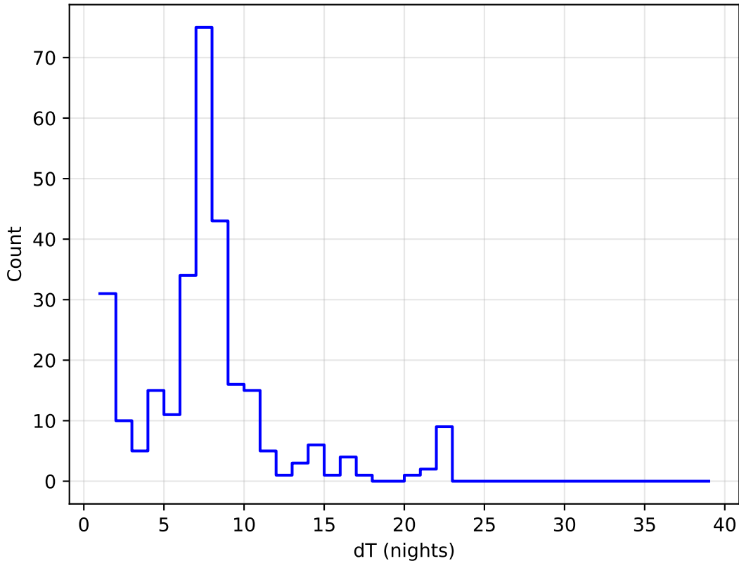
too_elab_r256_d3_gz_v3.4_10yrs all bands: DD:EDFS Delta Nights Histogram
