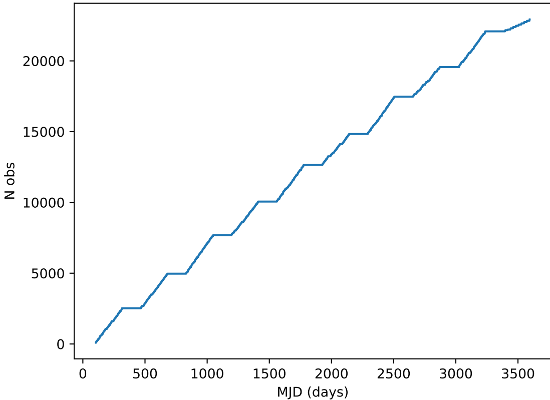
too_elab_r256_d3_gz_v3.4_10yrs all bands: DD:EDFS Cumulative NVisits
