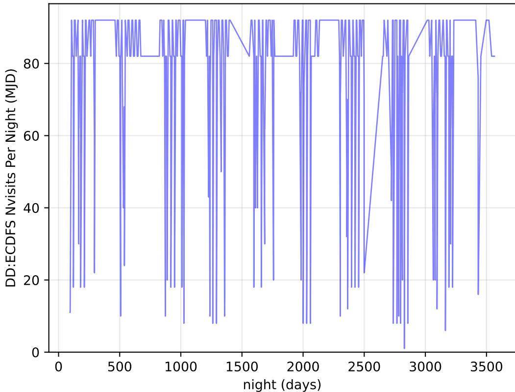
too_elab_r256_d3_gz_v3.4_10yrs all bands: DD:ECDFS Nvisits Per Night
