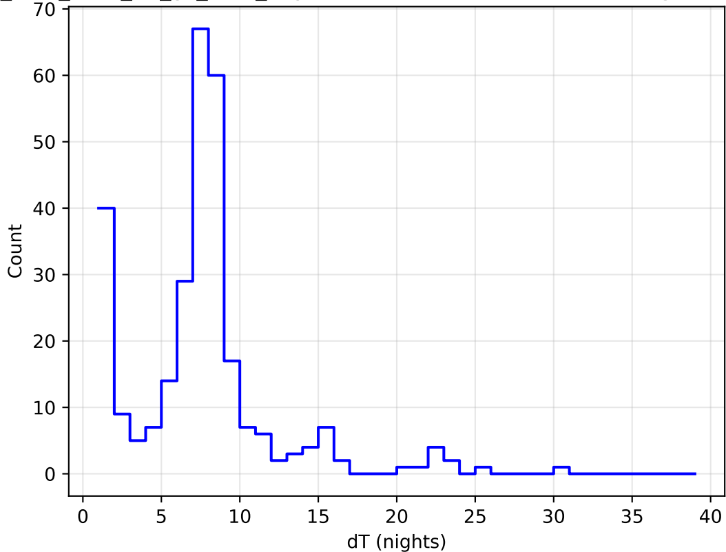
too_elab_r256_d3_gz_v3.4_10yrs all bands: DD:ECDFS Delta Nights Histogram
