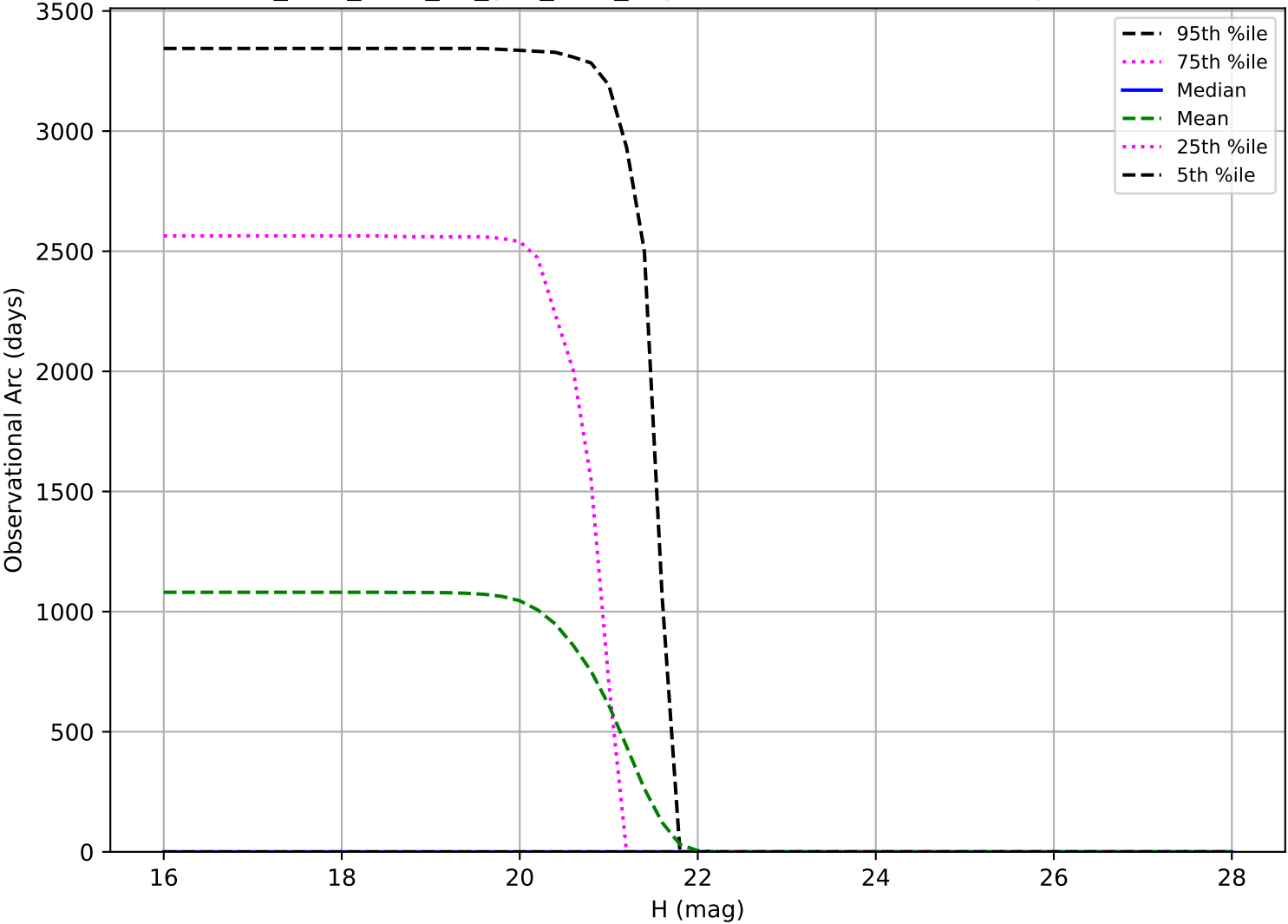
too_elab_r256_d3_griz_v3.4_10yrs: Observational Arc Length Vatra
