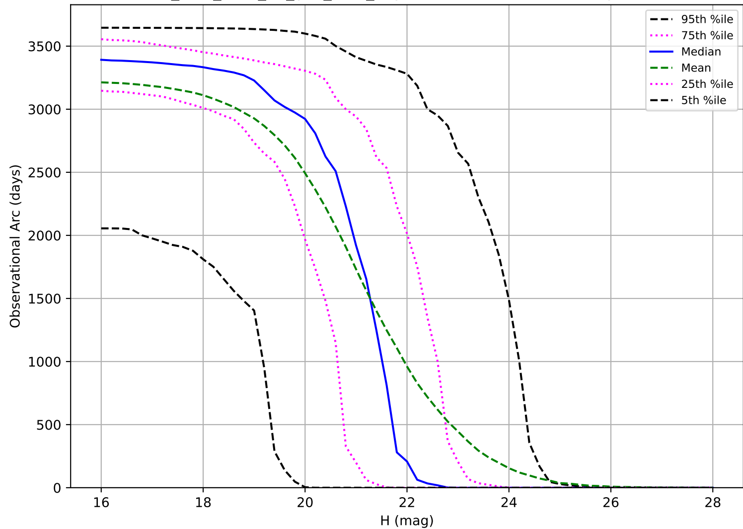
too_elab_r256_d3_griz_v3.4_10yrs: Observational Arc Length PHA
