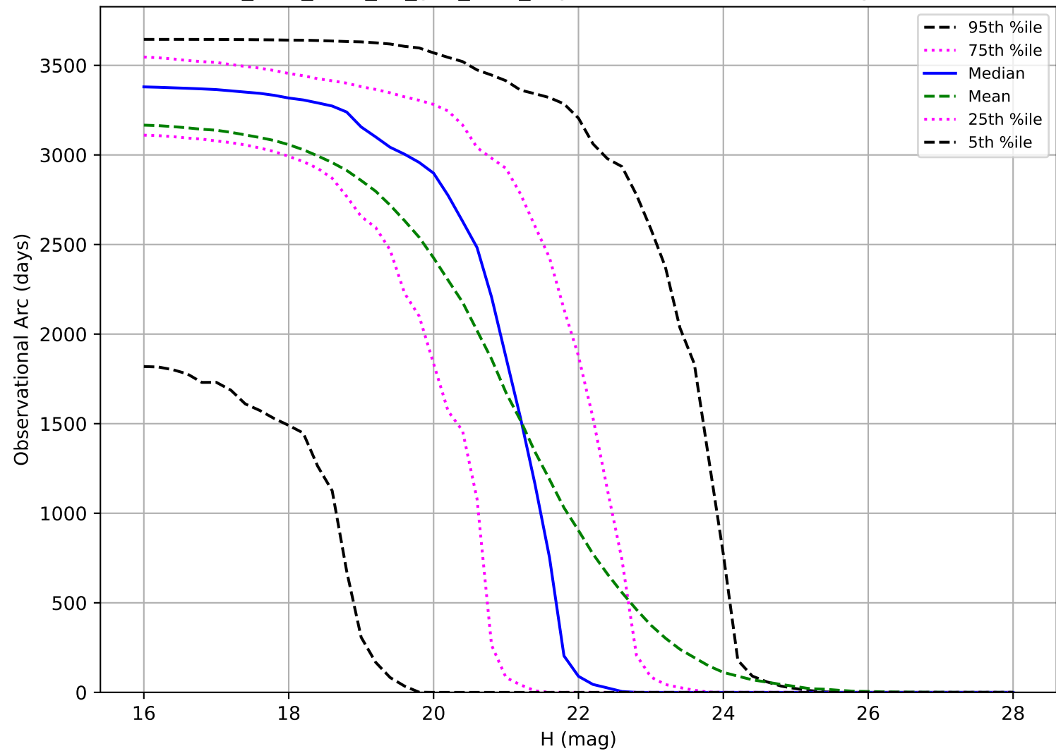
too_elab_r256_d3_griz_v3.4_10yrs: Observational Arc Length NEO
