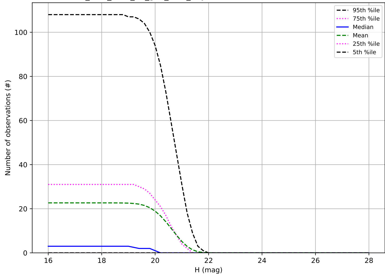
too_elab_r256_d3_griz_v3.4_10yrs: Number of observations Vatira
