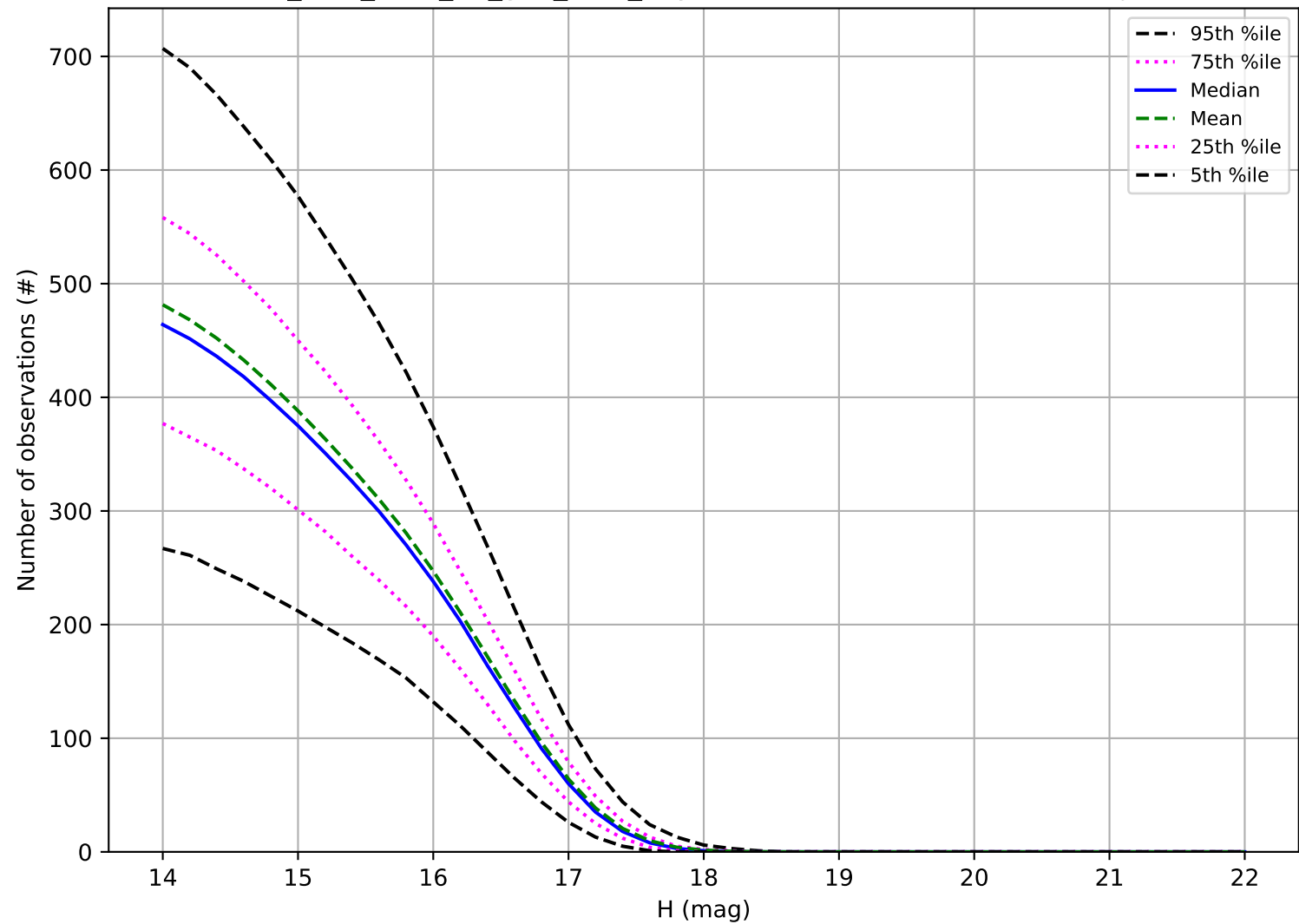
too_elab_r256_d3_griz_v3.4_10yrs: Number of observations Trojan
