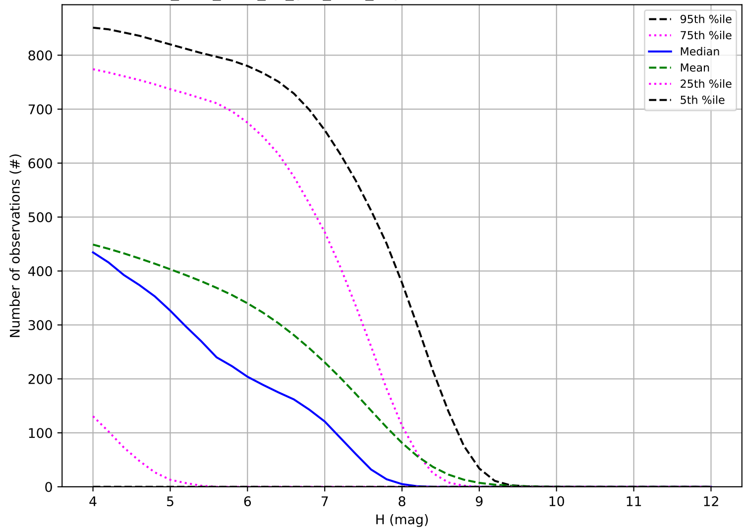
too_elab_r256_d3_griz_v3.4_10yrs: Number of observations TNO
