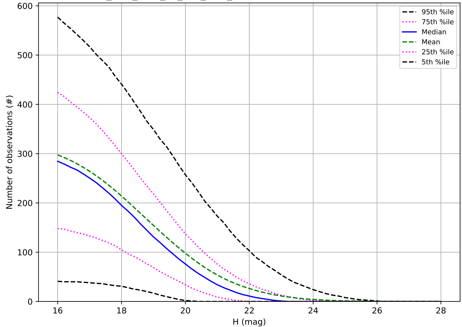
too_elab_r256_d3_griz_v3.4_10yrs: Number of observations PHA
