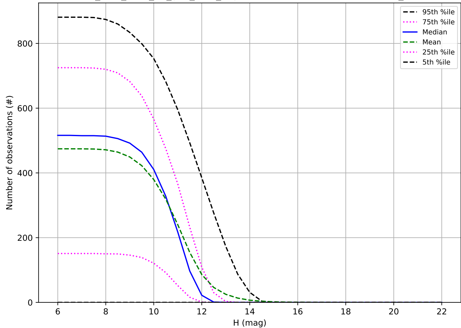
too_elab_r256_d3_griz_v3.4_10yrs: Number of observations OCC_r20
