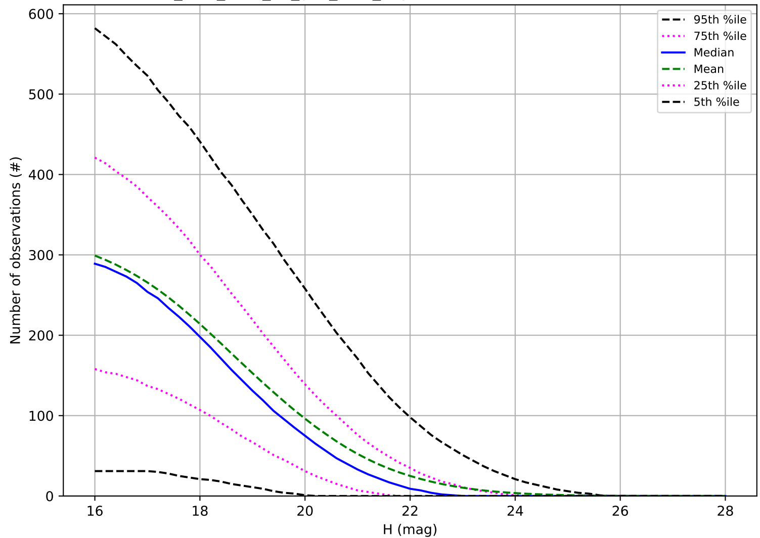
too_elab_r256_d3_griz_v3.4_10yrs: Number of observations NEO
