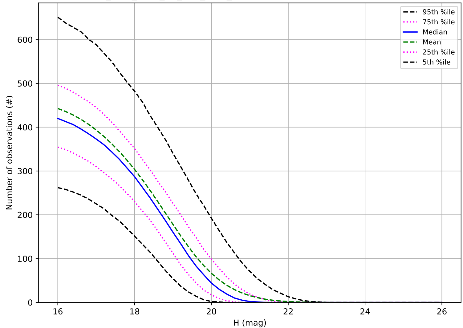
too_elab_r256_d3_griz_v3.4_10yrs: Number of observations MBA
