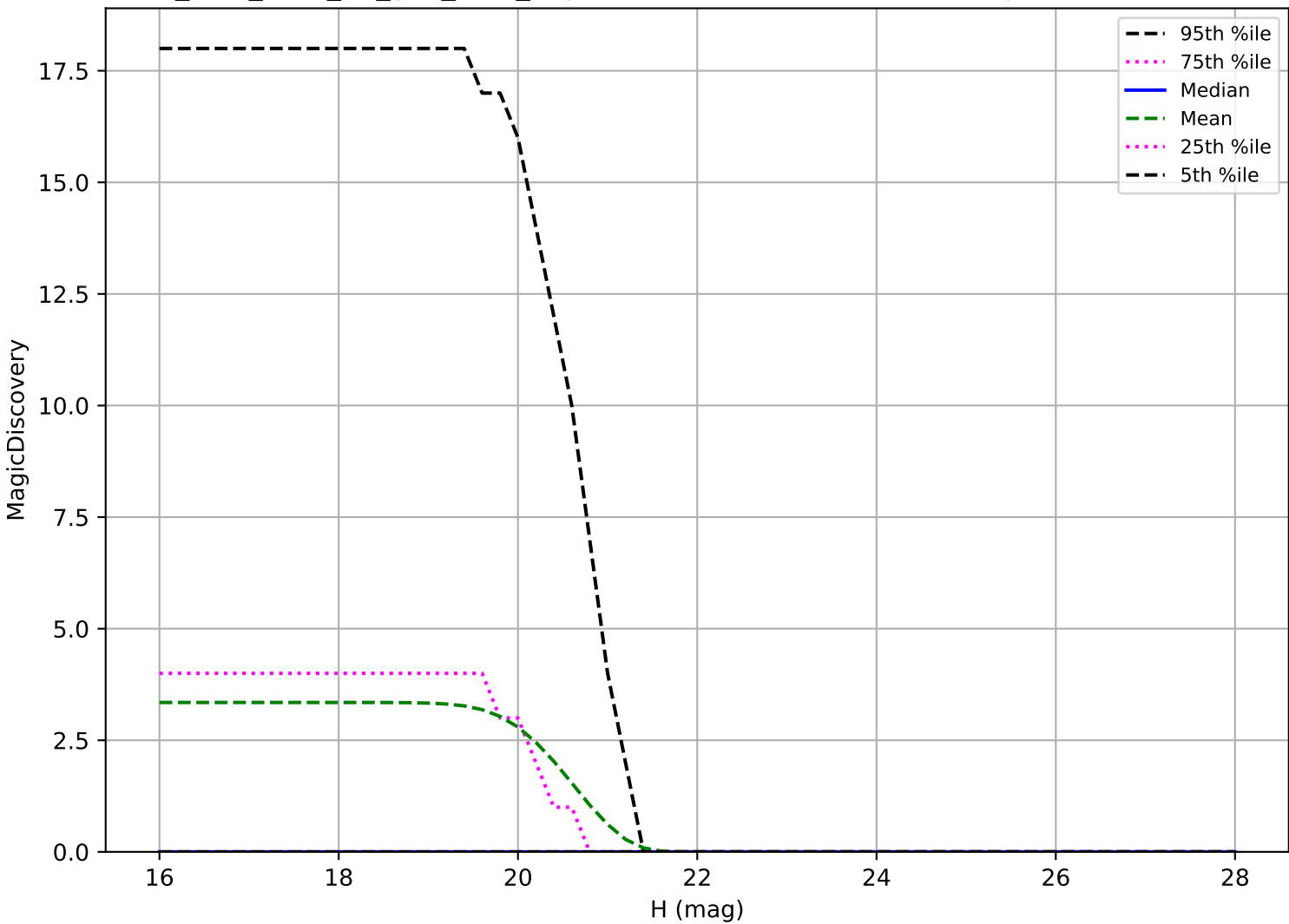
too_elab_r256_d3_griz_v3.4_10yrs: Vatira 6 detections in 60 nights detection loss
