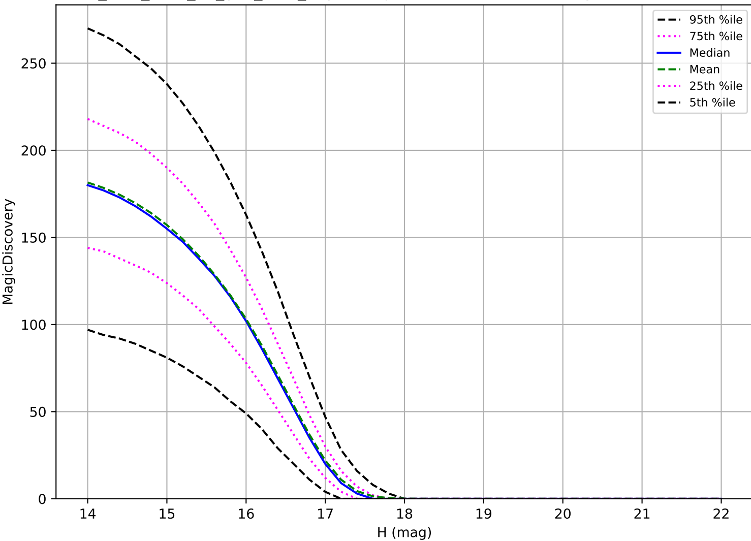
too_elab_r256_d3_griz_v3.4_10yrs: Trojan 6 detections in 60 nights detection loss
