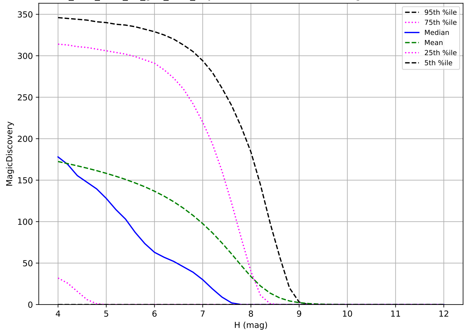
too_elab_r256_d3_griz_v3.4_10yrs: TNO 6 detections in 60 nights detection loss
