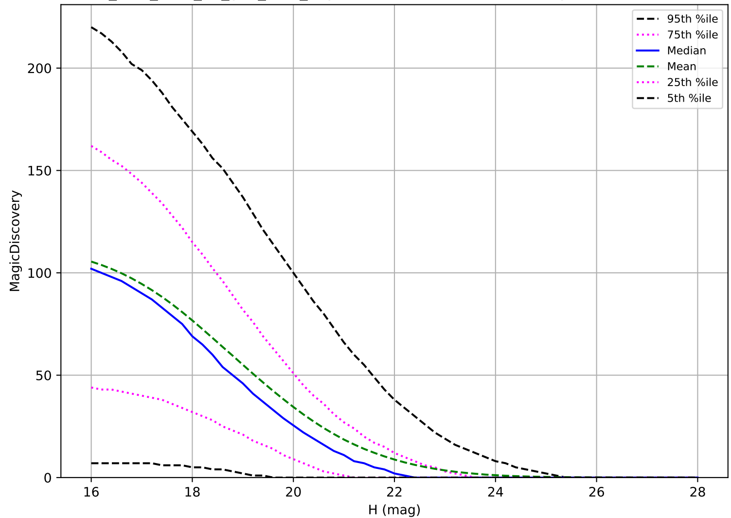
too_elab_r256_d3_griz_v3.4_10yrs: PHA 6 detections in 60 nights detection loss
