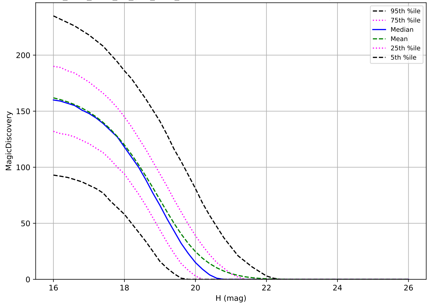
too_elab_r256_d3_griz_v3.4_10yrs: MBA 6 detections in 60 nights detection loss
