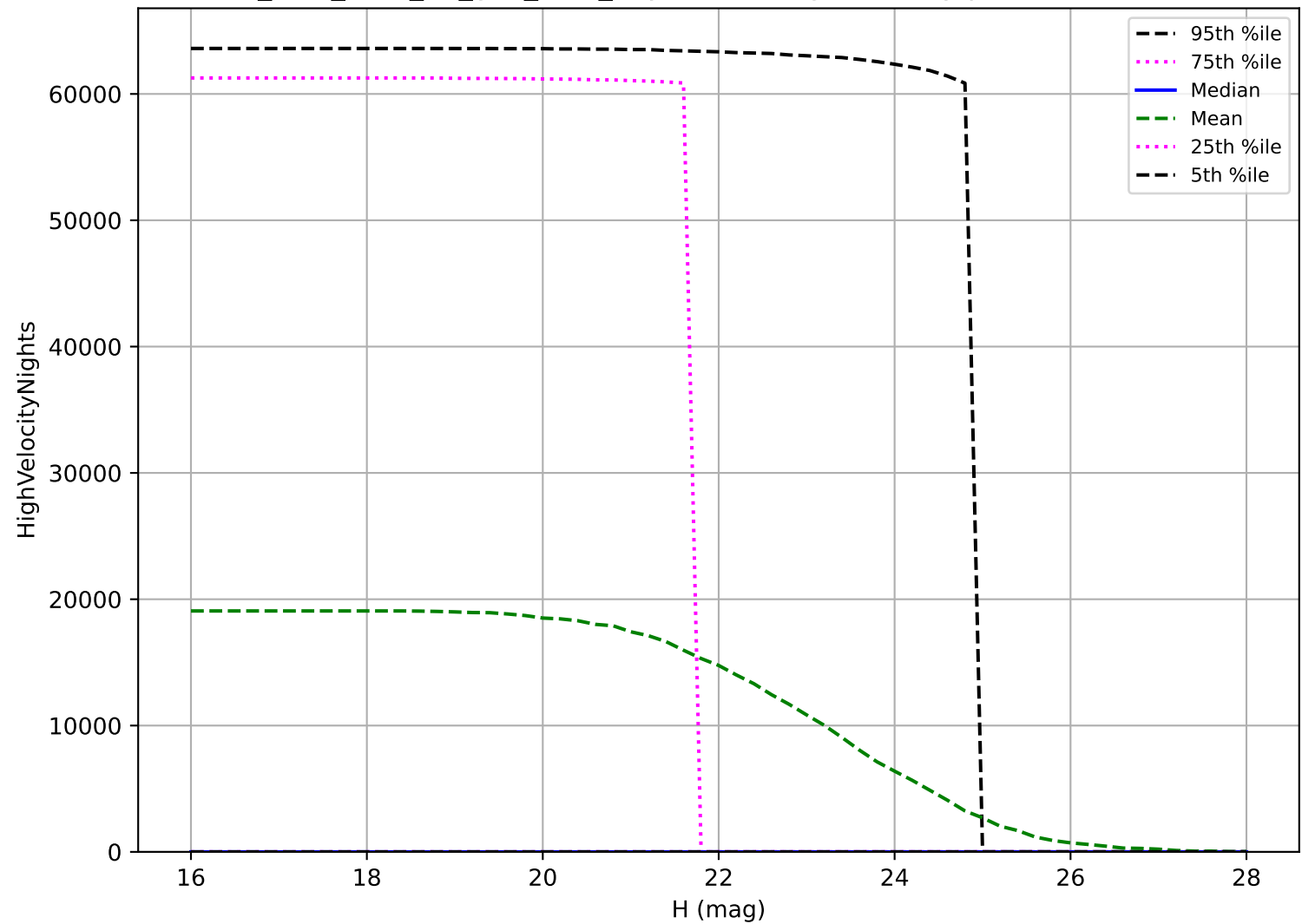
too_elab_r256_d3_griz_v3.4_10yrs: NEO High velocity pair detection loss
