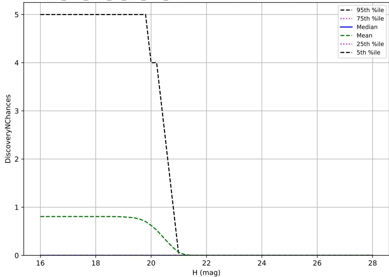
too_elab_r256_d3_griz_v3.4_10yrs: Vatira 3 pairs in 15 nights detection loss
