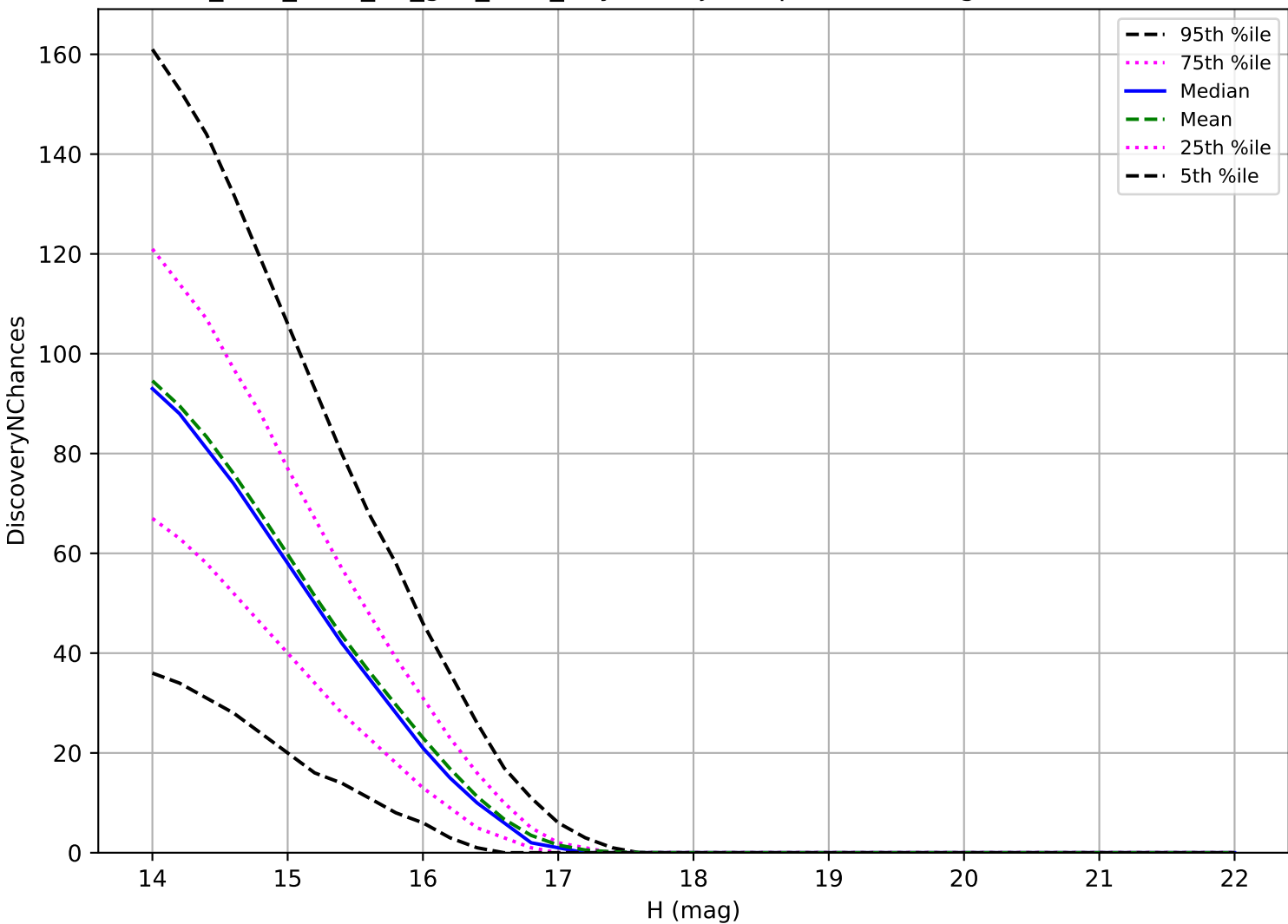
too_elab_r256_d3_griz_v3.4_10yrs: Trojan 3 pairs in 15 nights detection loss
