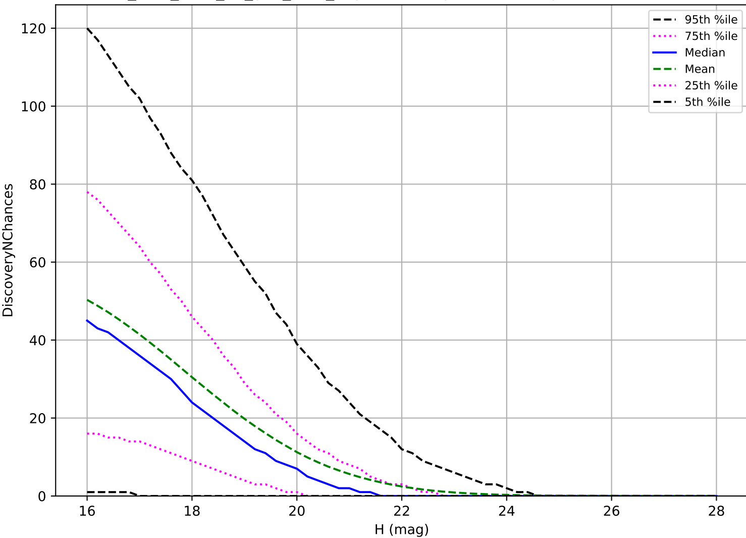
too_elab_r256_d3_griz_v3.4_10yrs: PHA 3 pairs in 15 nights detection loss
