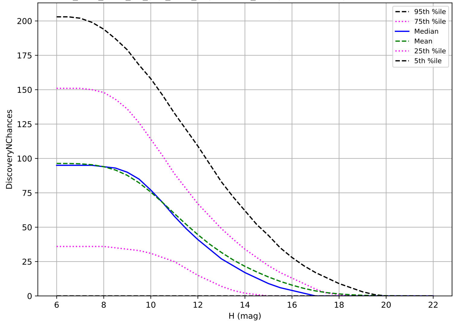
too_elab_r256_d3_griz_v3.4_10yrs: OCC_r5 3 pairs in 15 nights detection loss
