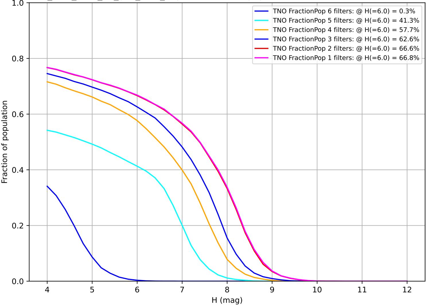
too_elab_r256_d3_griz_v3.4_10yrs: Fraction of population with colors in X filters TNO
