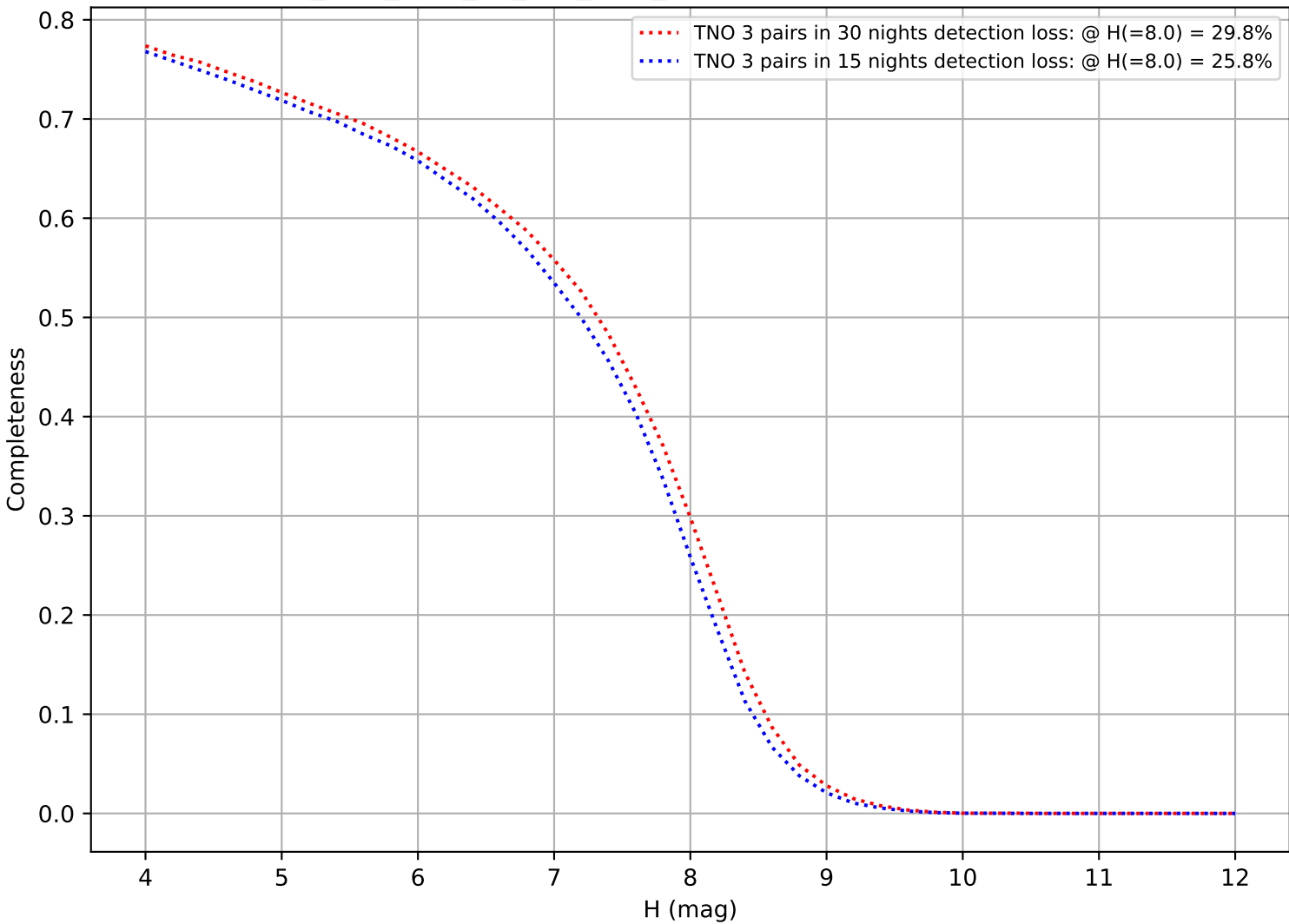
too_elab_r256_d3_griz_v3.4_10yrs: DifferentialCompleteness
