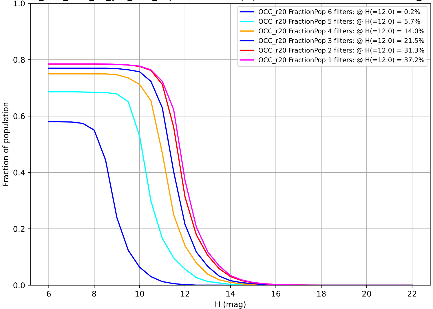
too_elab_r256_d3_griz_v3.4_10yrs: Fraction of population with colors in X filters OCC_r20
