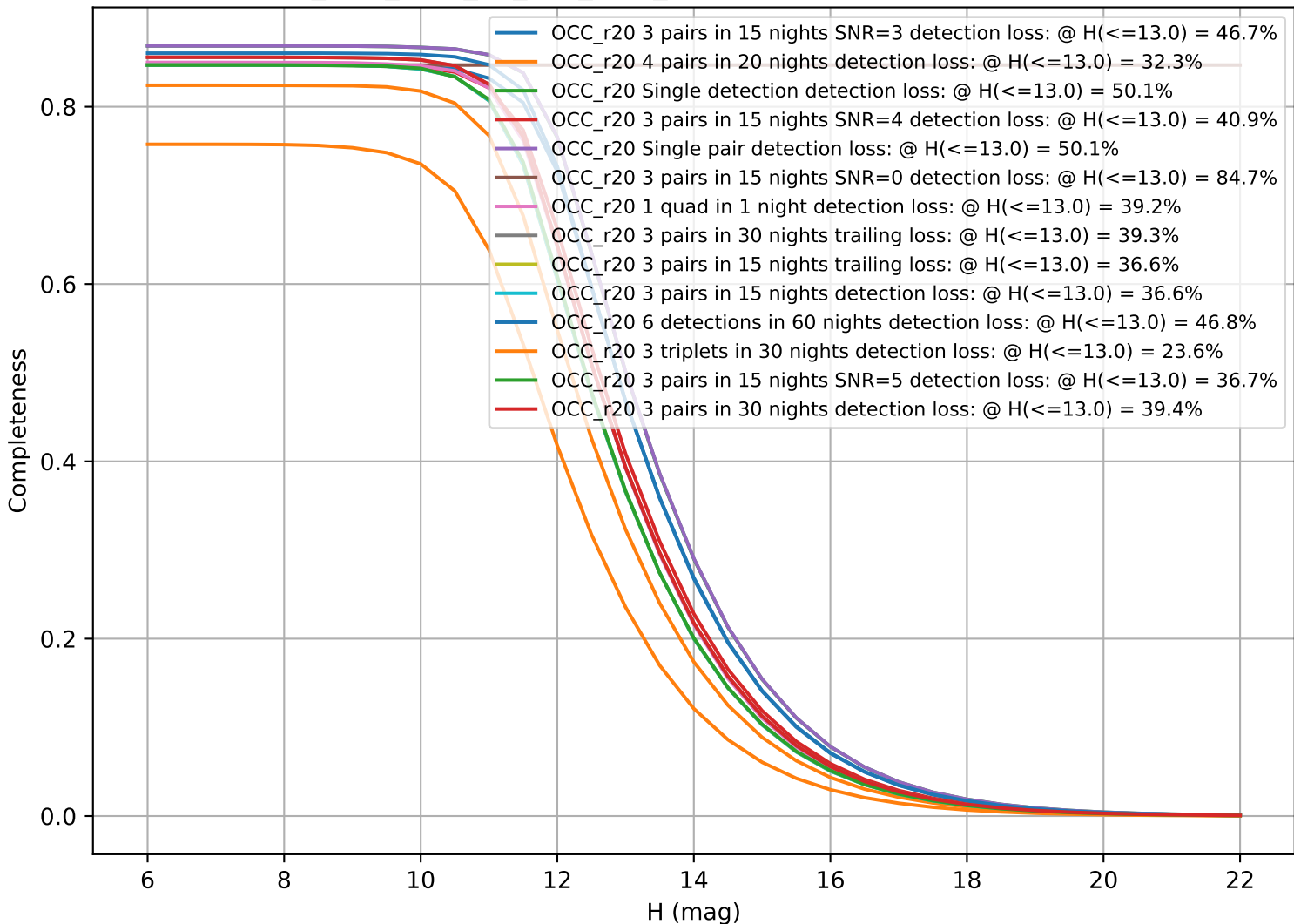
too_elab_r256_d3_griz_v3.4_10yrs: CumulativeCompleteness
