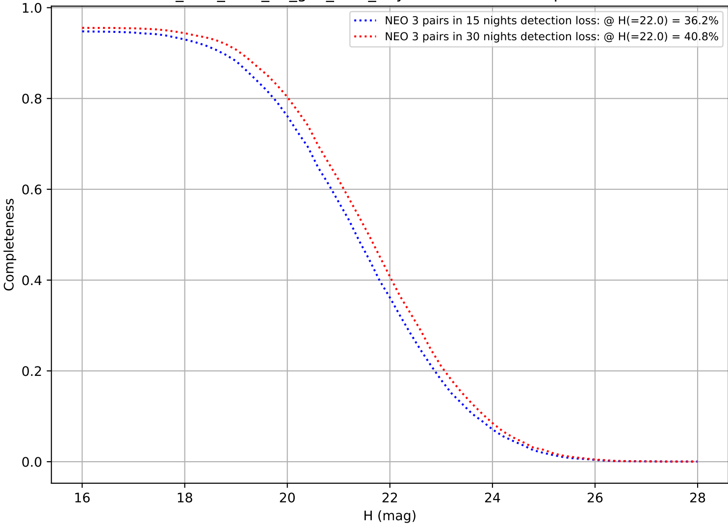
too_elab_r256_d3_griz_v3.4_10yrs: DifferentialCompleteness
