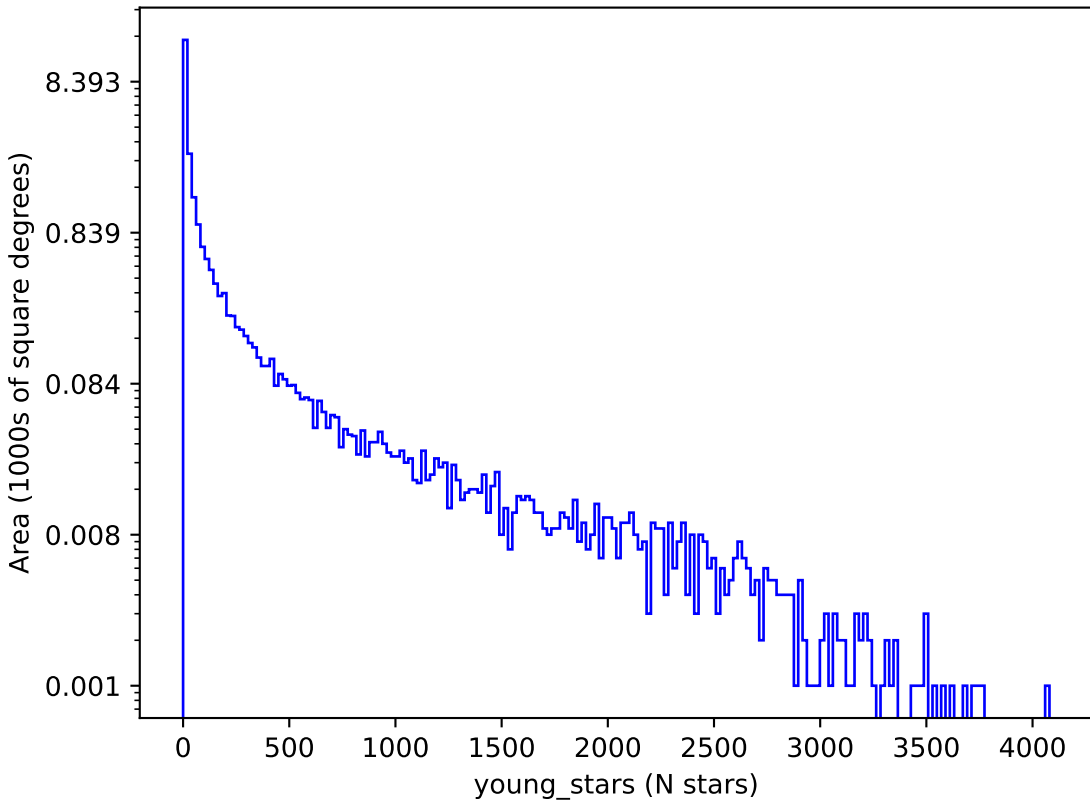
too_elab_r256_d3_griz_v3.4_10yrs : young_stars
