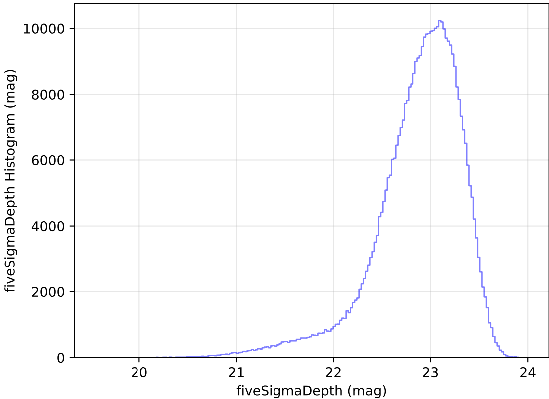
too_elab_r256_d3_griz_v3.4_10yrs z: fiveSigmaDepth Histogram
