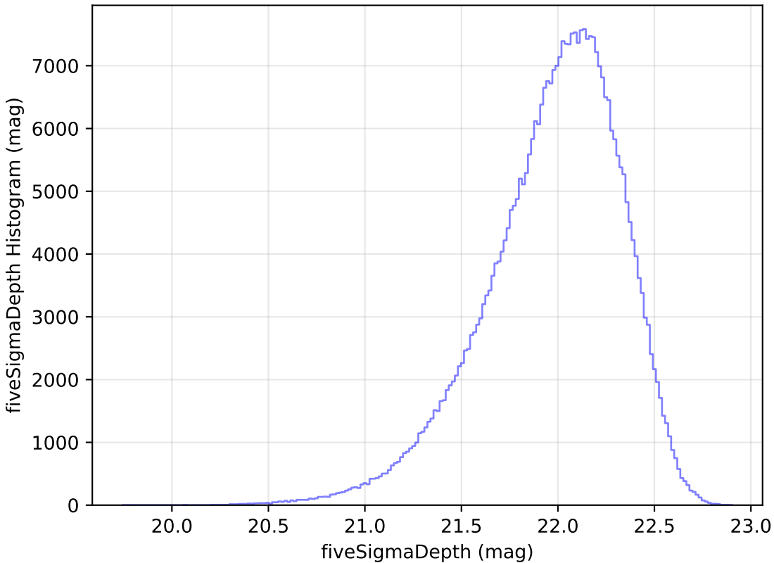
too_elab_r256_d3_griz_v3.4_10yrs y: fiveSigmaDepth Histogram
